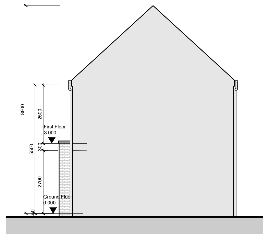
Side Elevation 02
