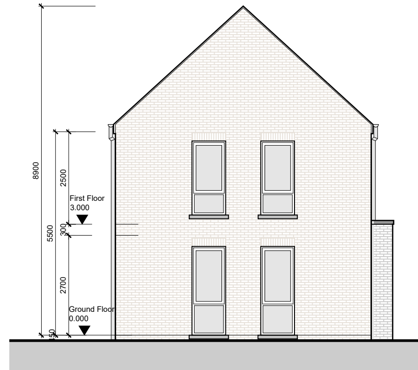
Side Elevation 01
