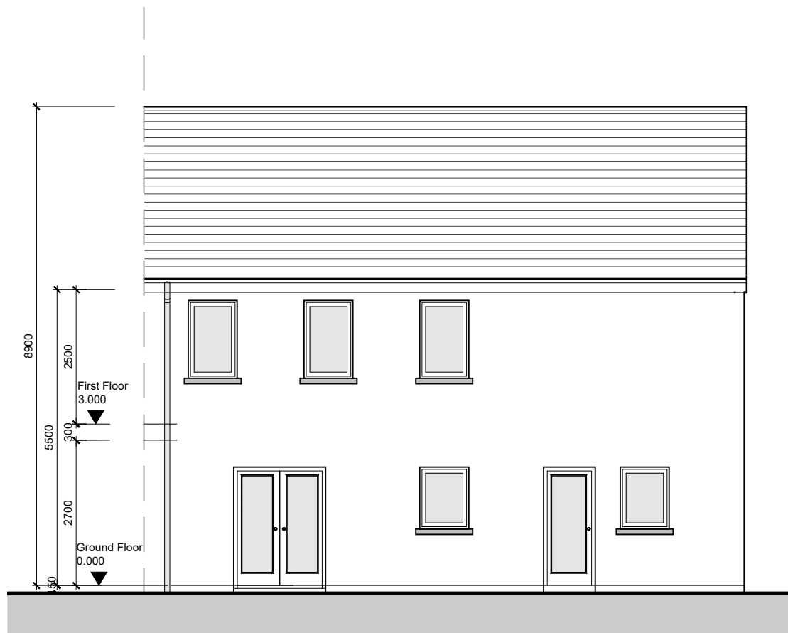
Rear Elevation
